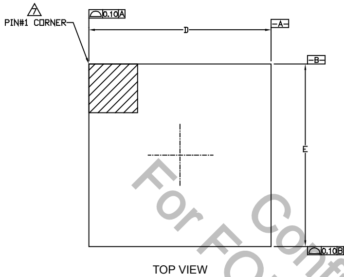
Figure 5-1. Top View of the A12A35 Package.
