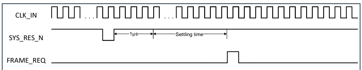
Figure 23: Reset Sequence
