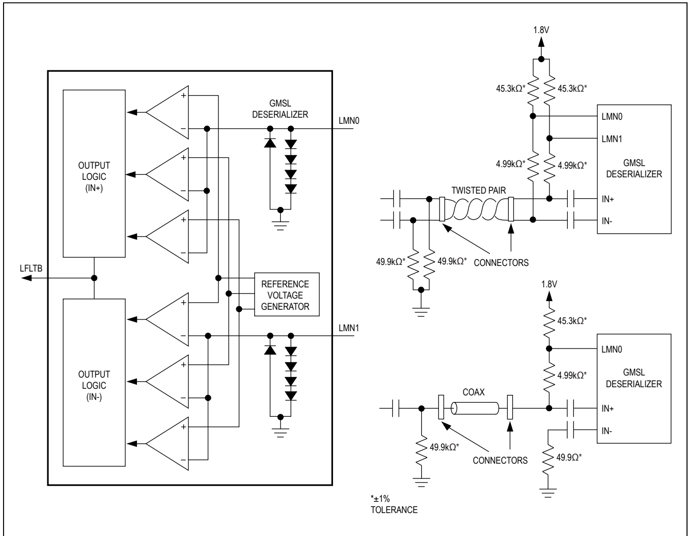
Figure 4. Line Fault
