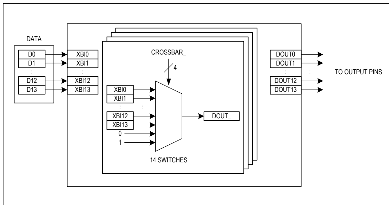
Figure 18. Crosspoint-Switch Dataflow
