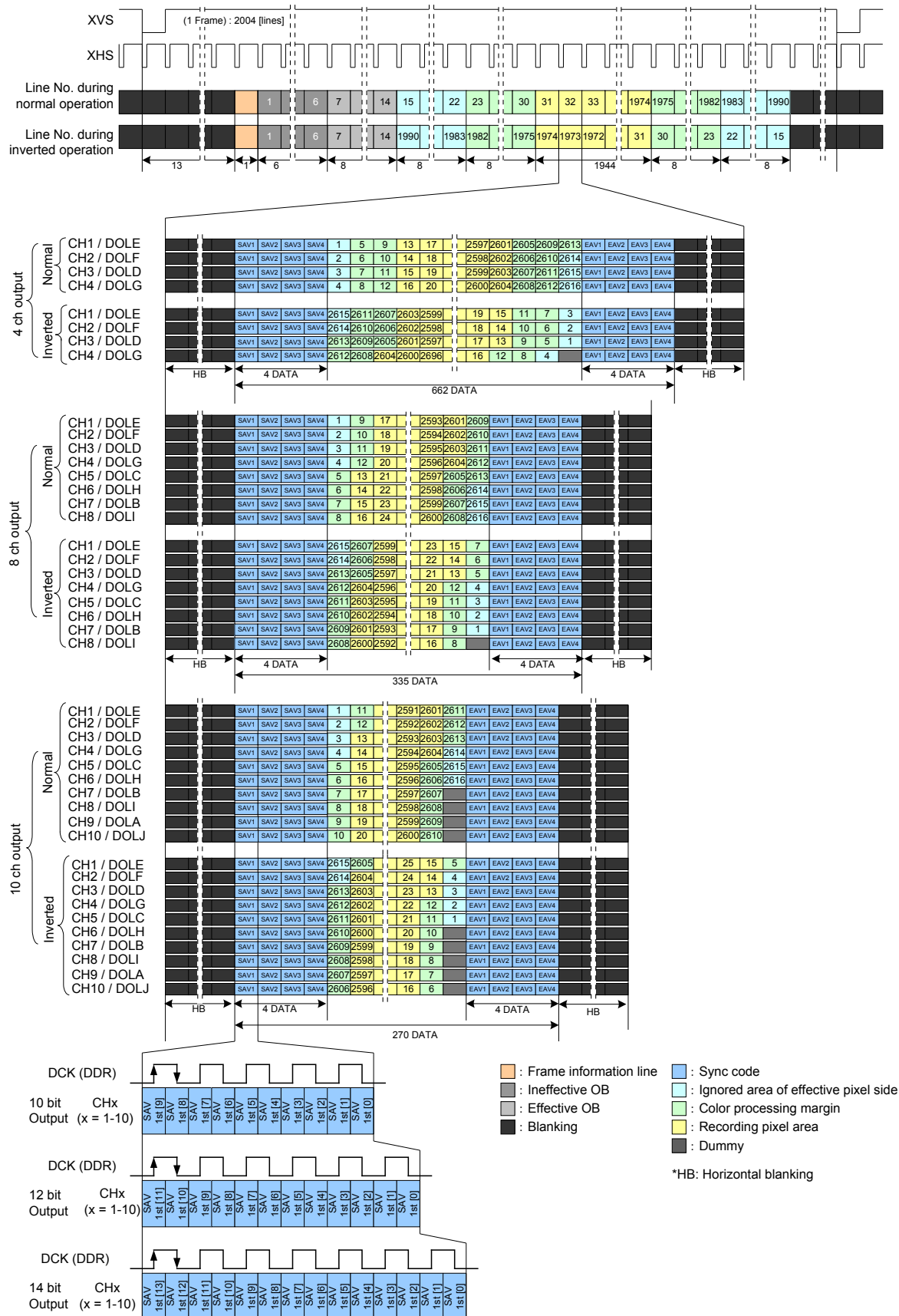
Drive Timing Chart for Window cropping 5.0 M (4:3) Mode
