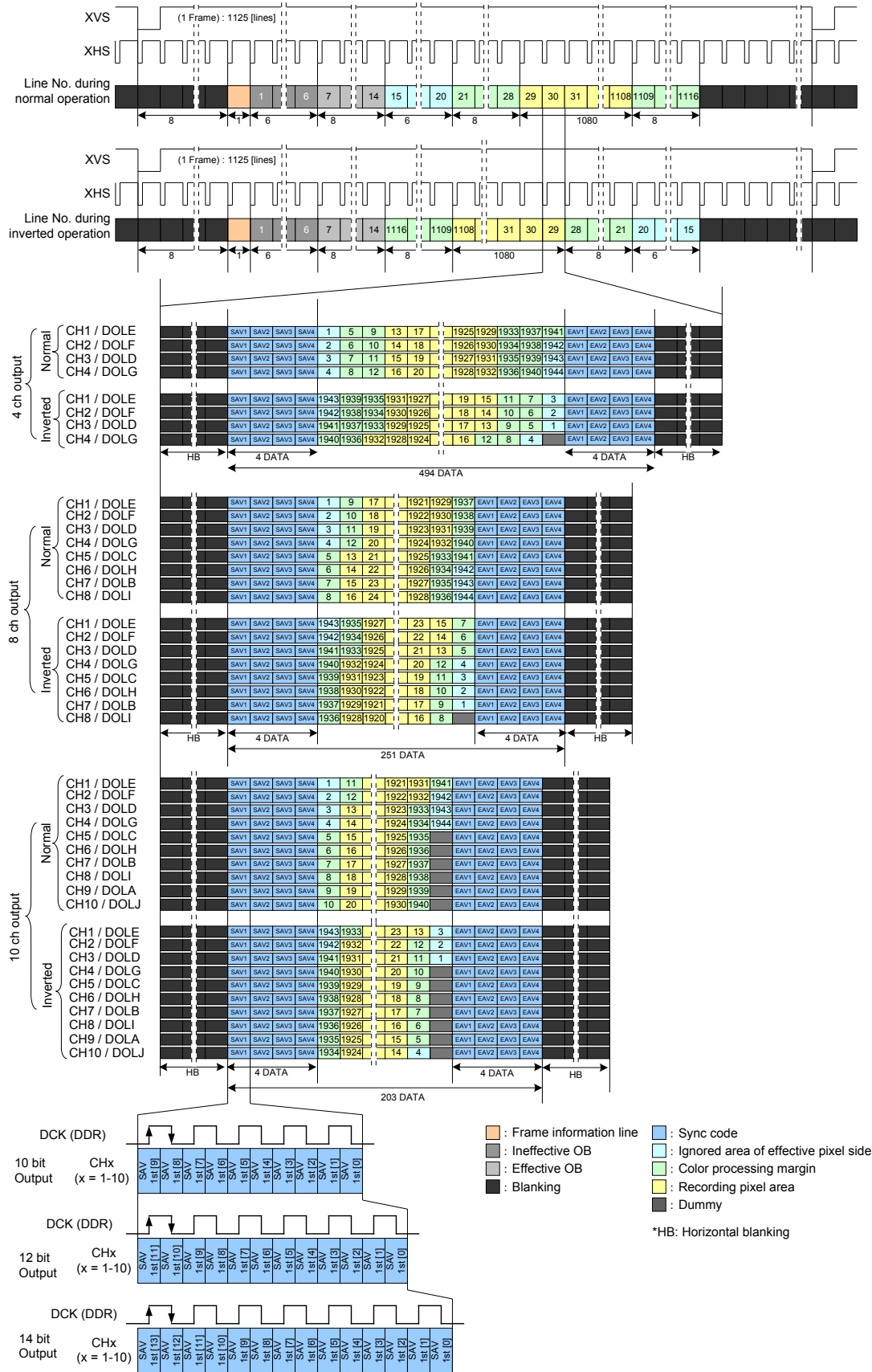
Drive Timing in HD 1080p Mode
