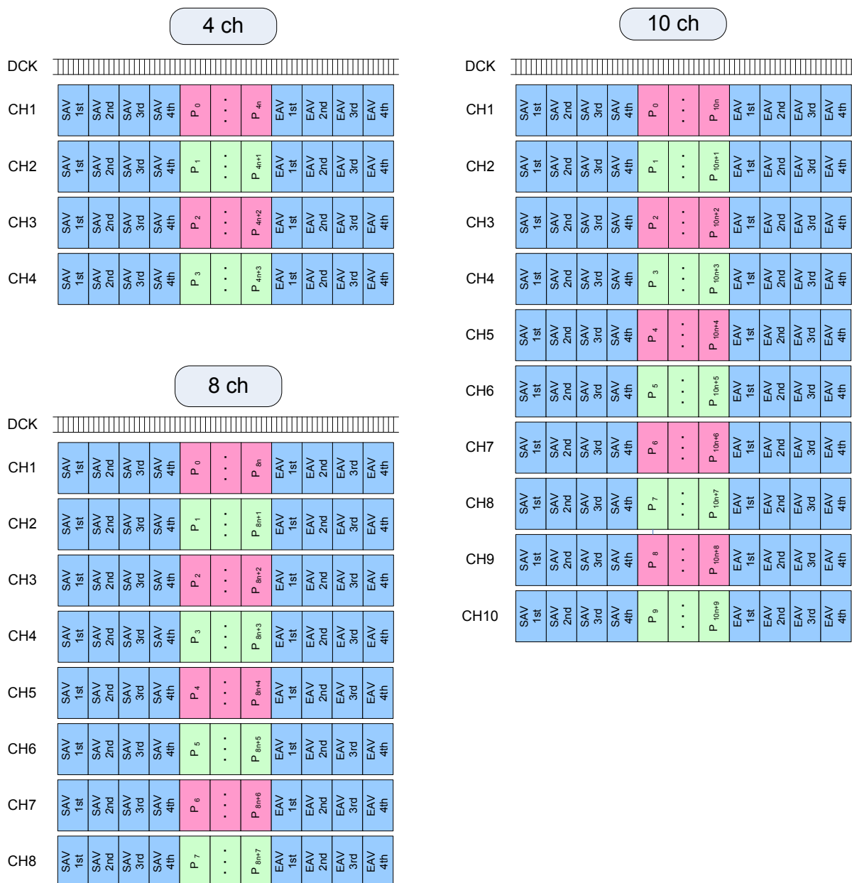
Low-voltage LVDS Serial 4 ch / 8 ch / 10 ch Output Format
