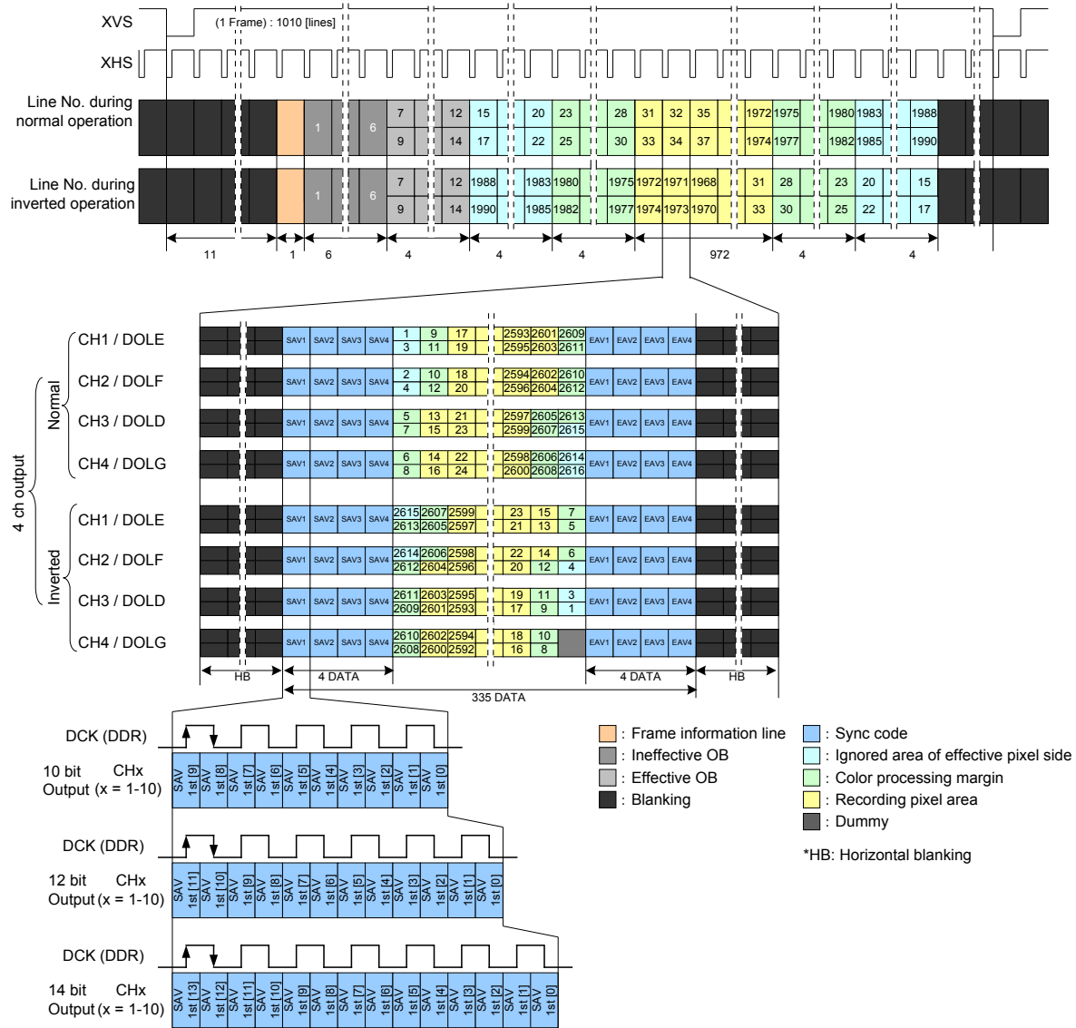
Drive Timing Chart for Window cropping 1.3 M (4:3) 2 x 2 Binning Mode
