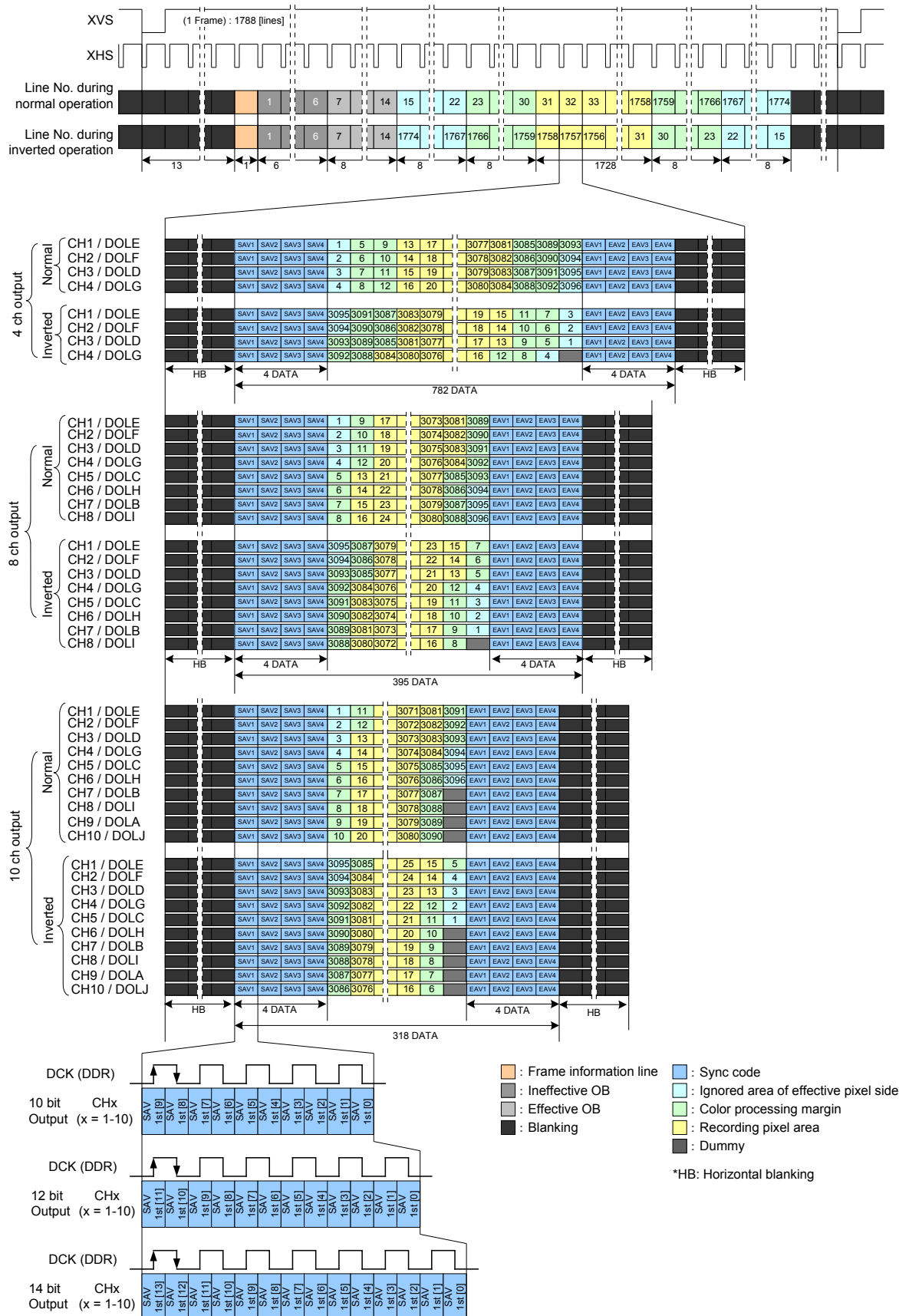
Drive Timing Chart for Window cropping 5.3 M (16:9) Mode
