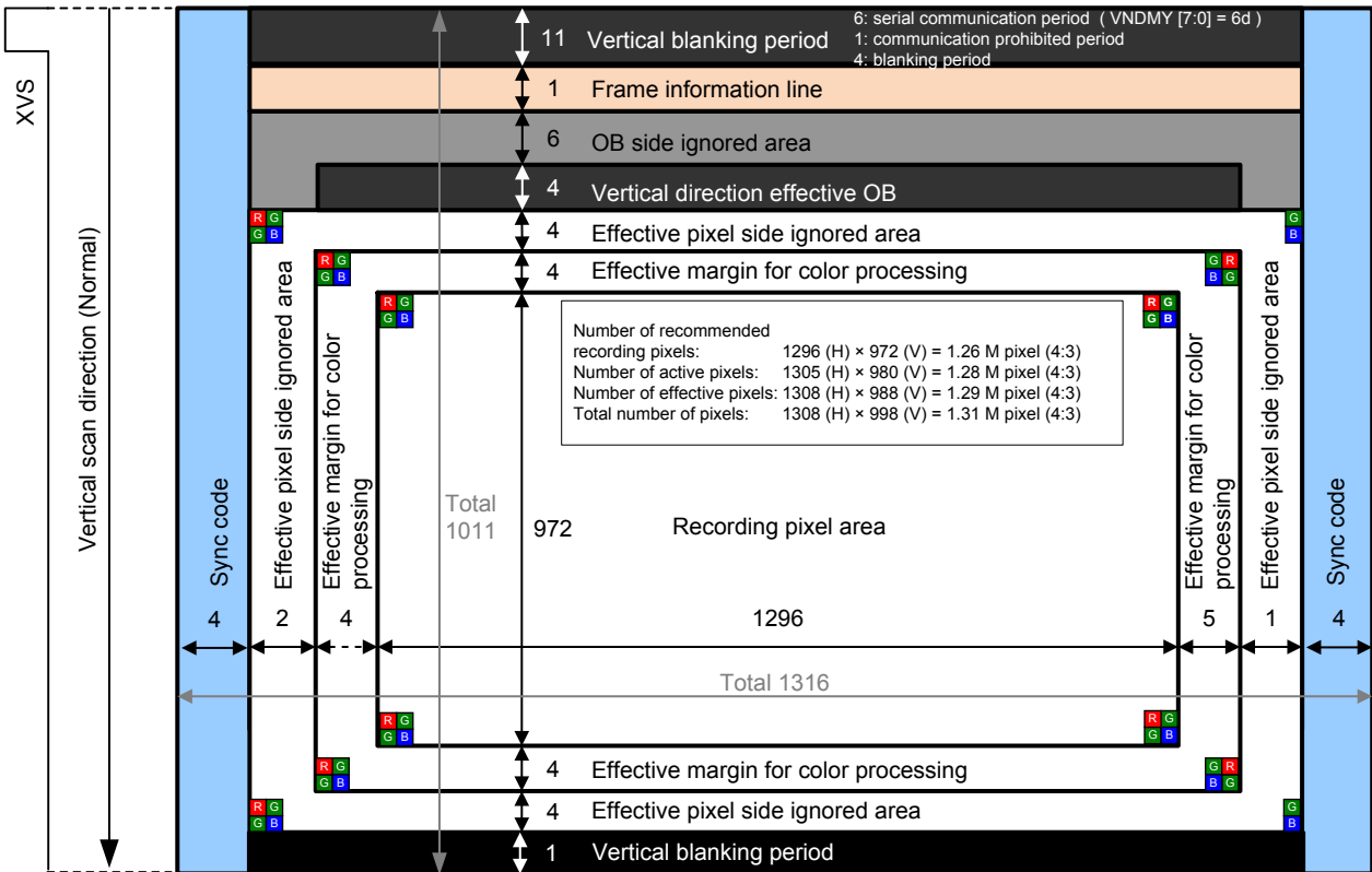
Pixel Array Image in Window cropping 1.3 M (4:3) 2 × 2 Binning Mode
