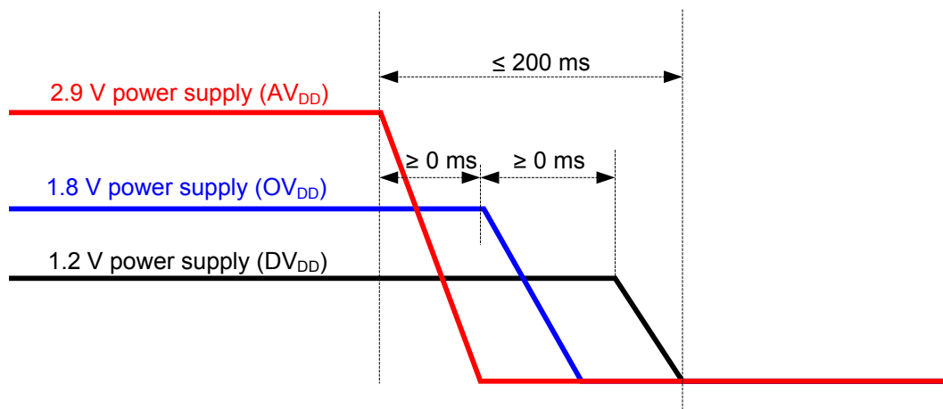
Power-off Sequence
