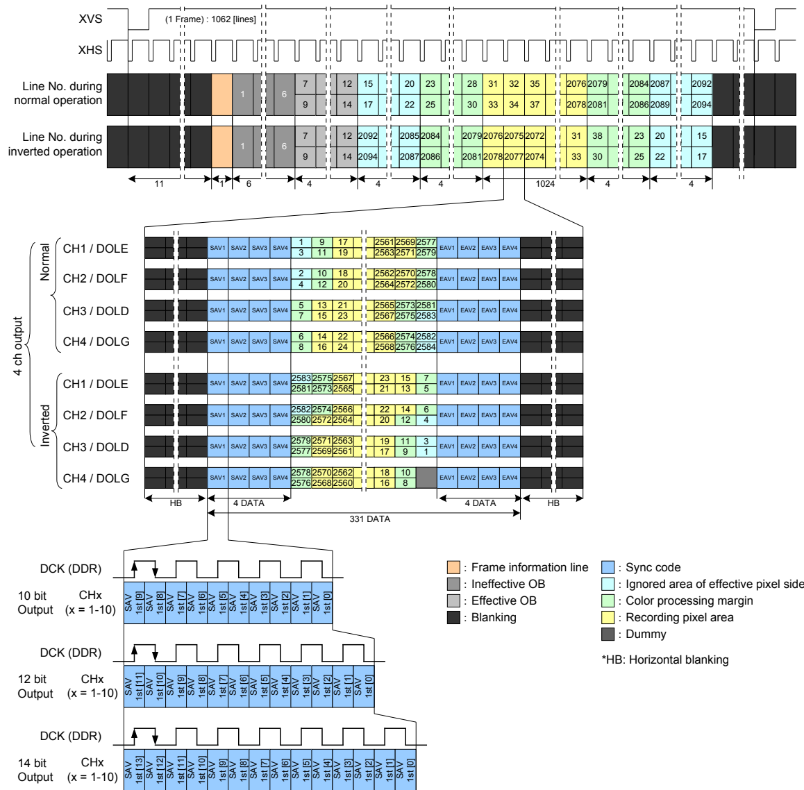
Drive Timing Chart for Window cropping 1.3 M (5:4) QSXGA 2 × 2 Binning Mode
