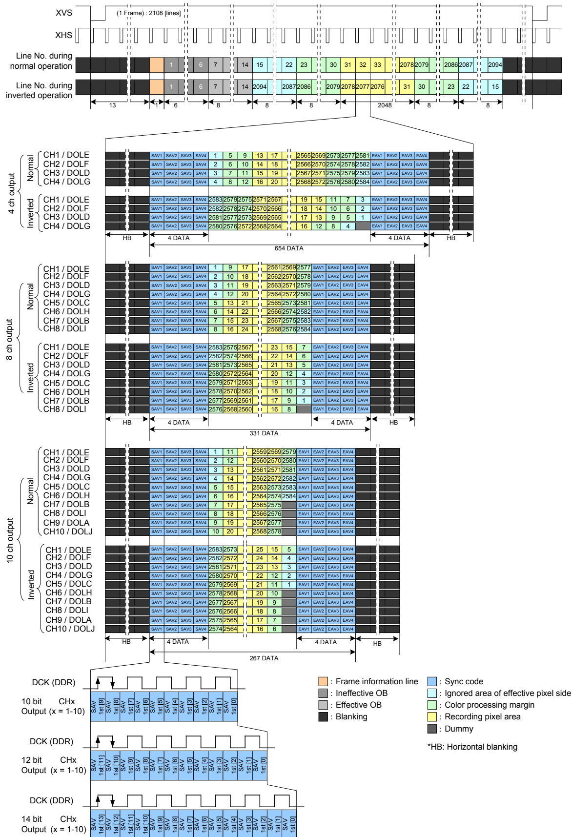
Drive Timing Chart for Window cropping 5.2 M (5:4) QSXGA Mode
