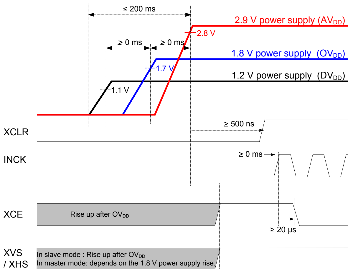
Power-on Sequence
