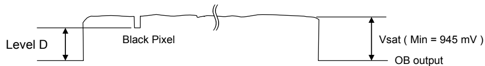
Signal output waveform of R/G/B channel
