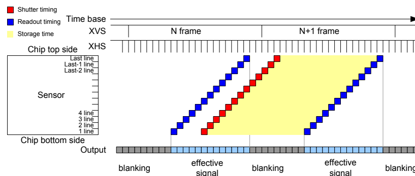
Image Drawing of Shutter Operation
