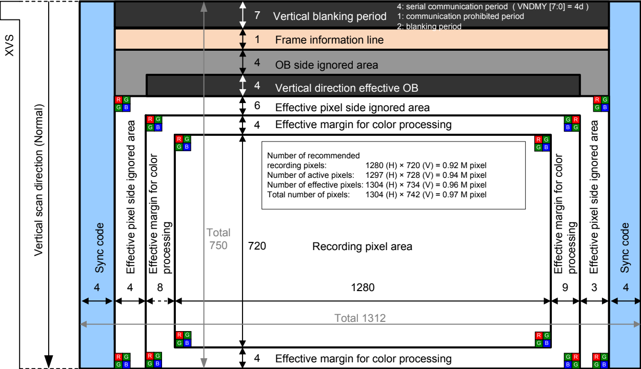
Pixel Array Image in HD 720p 2 x 2 Binning Mode
