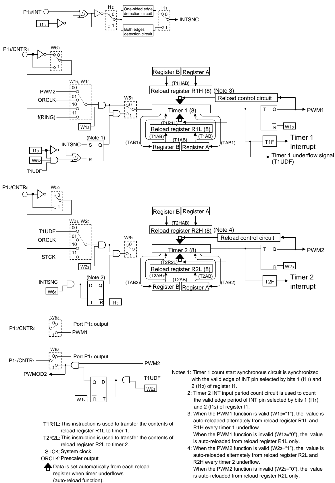
Fig. 23 Timers structure (2)
