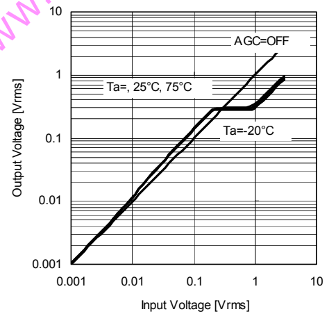
AGC Output Voltage vs. Input Voltage V_+=9\text{V} , R_L=47\text{k}\Omega , V_{in}(\text{A+Bch}) , f=1\text{kHz} , V_{out}(\text{Ach}) , \text{BW}=400\text{Hz}-30\text{kHz} , \text{VOL}=0\text{dB} , \text{BAL}=0\text{dB} , \text{AGC}=300\text{mV} , \text{BASS}=\text{TREB}=0\text{dB} , \text{BBE}=\text{OFF} , \text{Surround}=\text{OFF}
