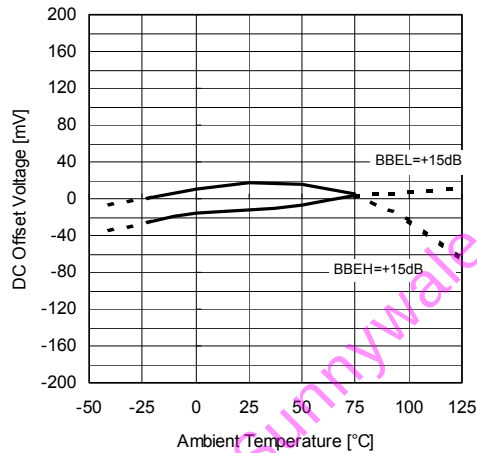
DC Offset Voltage vs. Ambient Temperature (BBE)
