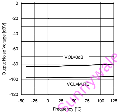
Output Noise Voltage (LINE) vs. Frequency V_+=9\text{V} , R_L=47\text{k}\Omega , \text{BAL}=0\text{dB} , \text{AGC}=\text{OFF} , \text{BASS}=\text{TREB}=0\text{dB} , \text{BBE}=\text{OFF} , \text{Surround}=\text{OFF}
