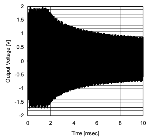
AGC Attack Time Response T_a=25^{\circ}\text{C} , V_+=9\text{V} , R_L=47\text{k}\Omega , V_{in}(\text{A+Bch}) , f=20\text{kHz} , V_{out}(\text{Ach}) , \text{BW}=400\text{Hz}-30\text{kHz} , \text{VOL}=0\text{dB} , \text{BAL}=0\text{dB} , \text{AGC}=300\text{mV} , \text{BASS}=\text{TREB}=0\text{dB} , \text{BBE}=\text{OFF} , \text{Surround}=\text{OFF}
