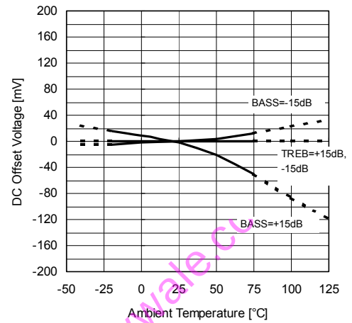
DC Offset Voltage vs. Ambient Temperature (Surround)
