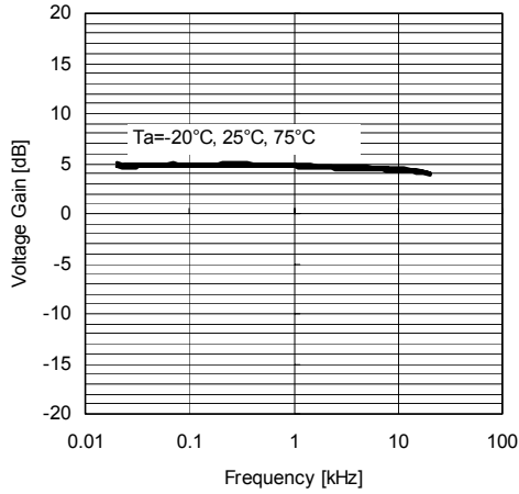
Voltage Gain (LINE) vs. Frequency T_a=25^{\circ}\text{C} , V_+=9\text{V} , R_L=47\text{k}\Omega , V_{in}(\text{Ach})=0.1\text{Vrms} , V_{out}(\text{LINEAch}) , \text{VOL}=0\text{dB} , \text{BAL}=0\text{dB} , \text{AGC}=\text{OFF} , \text{BASS}=\text{TREB}=0\text{dB} , \text{BBE}=\text{OFF} , \text{Surround}=\text{OFF}
